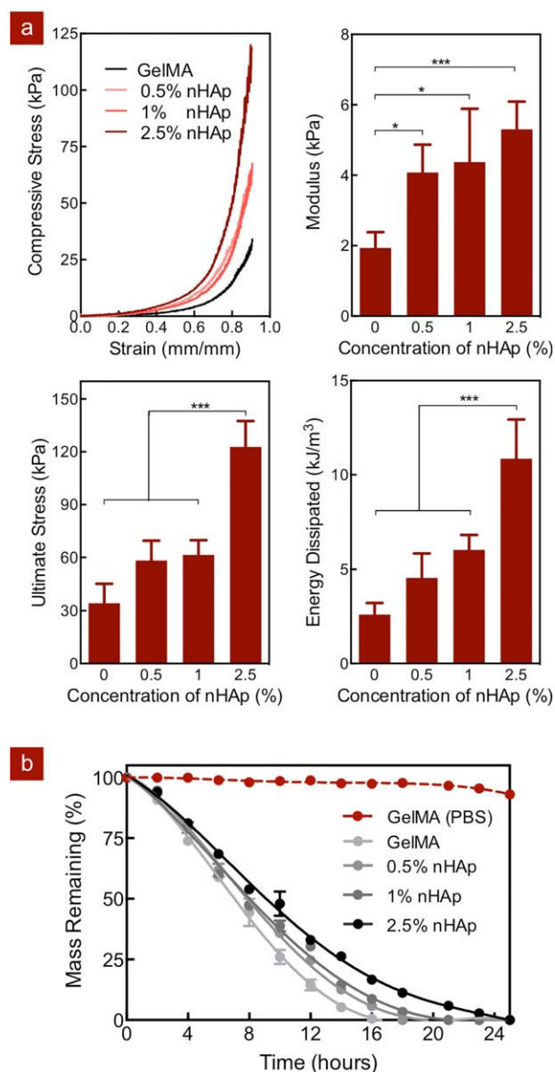
FIGURE 4. The effect of nHAp on the mechanical stiffness and physiological stability of nanocomposite hydrogels. (a) The stress-strain curve indicates increase in modulus, ultimate stress and energy dissipated due to addition of nHAp. (b) The degradation rate of nanocomposite hydrogel decreases with the addition of nHAp.
