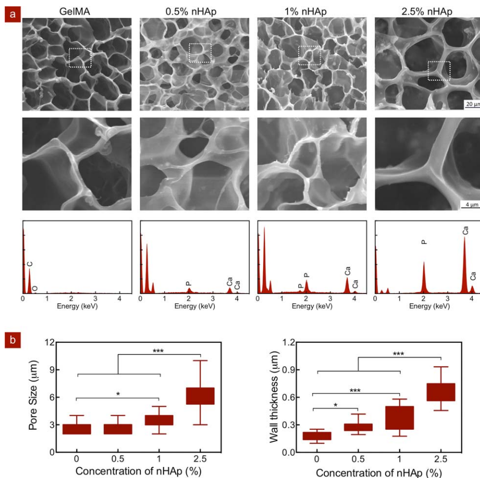
FIGURE 3. The effect of nHAp in nanocomposite network. (a) All the hydrogels exhibit porous and interconnected networks. The addition of nHAp results in formation of a hydrogel network with larger pore size. EDS spectra indicate presence of Ca and P in the nanocomposite network. (b) The effect of nHAp addition on pore size and pore wall thickness in the polymer network was quantified using ImageJ.
